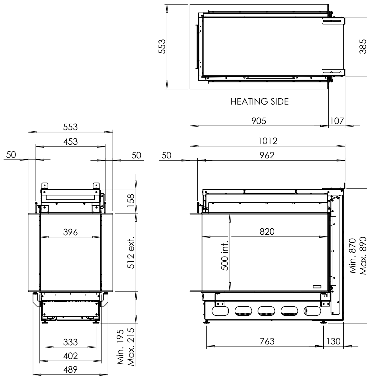
Dimensional Drawing e-MatriX Mood 800/500 RD
