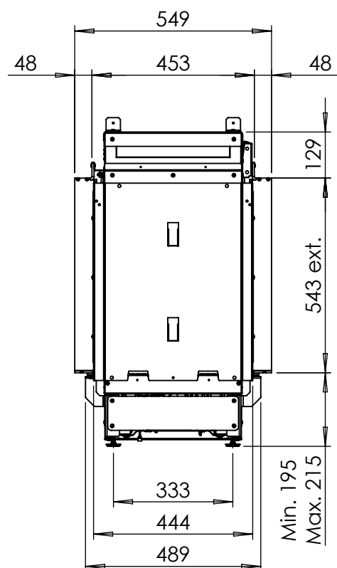
Dimensional Drawing e-MatriX Mood 800/500 ST
