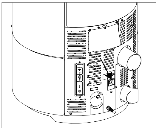
ELECTRICAL STOVE CONNECTION
