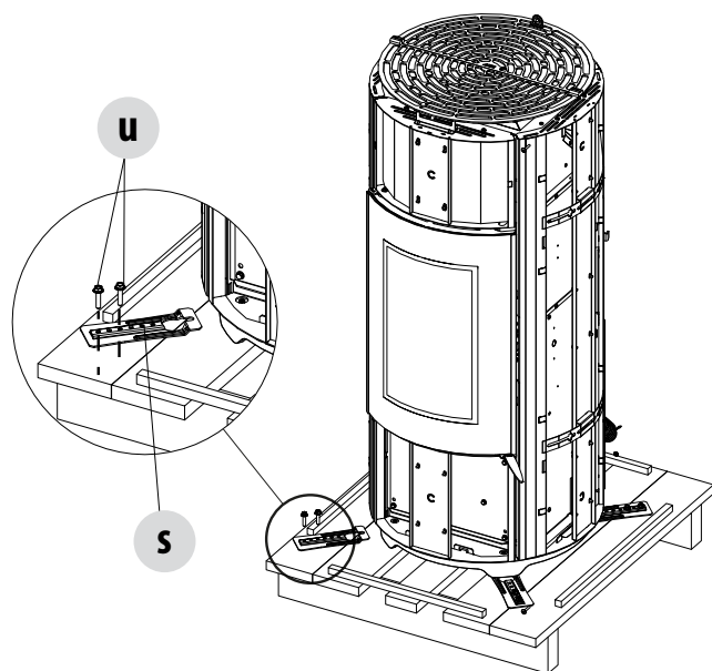
REMOVING FASTENING BRACKETS
