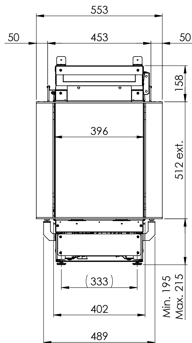
Dimensional drawing e-Matrix 800/500-RD-RGB
