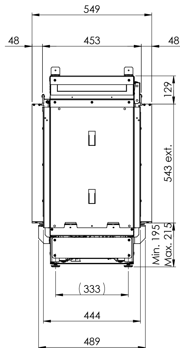
Dimensional drawing e-Matrix 800/500-ST-RGB
