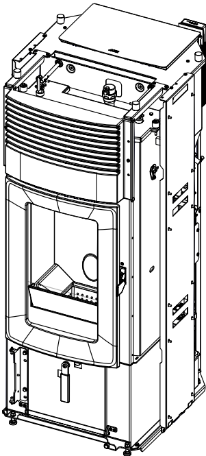
STOVE STRUCTURE
