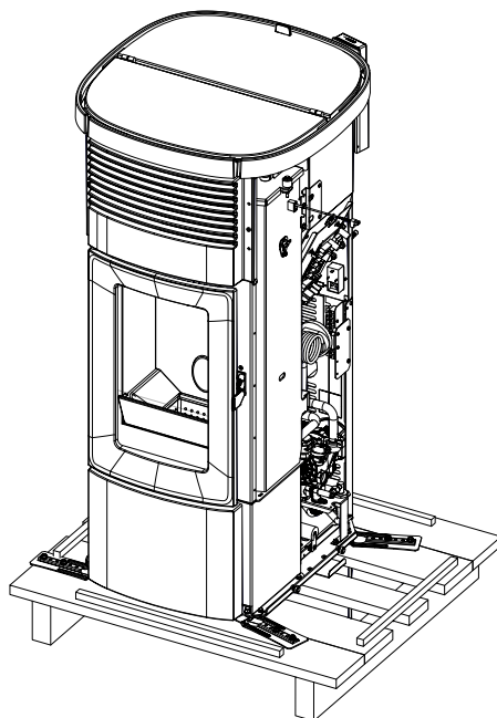
REMOVING THE FASTENING BRACKETS (MUSA STOVES)
